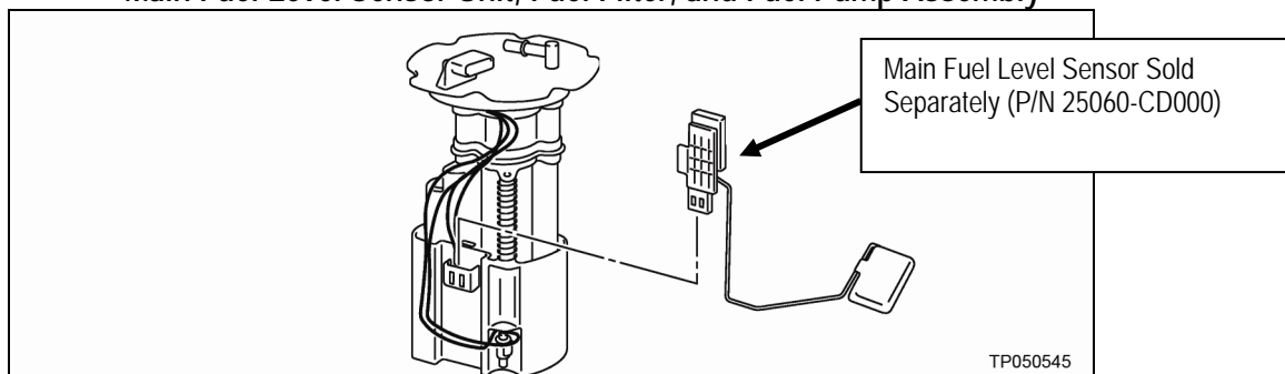
Main Fuel Level Sensor Unit, Fuel Filter, and Fuel Pump Assembly
