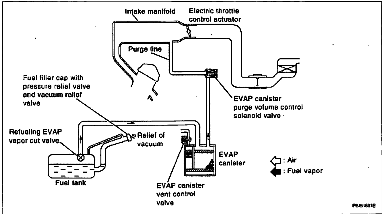
Fig 5: Evaporative Emission System Diagram
